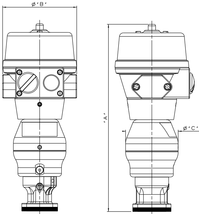
DN15 S360 ø50 PISTON SPRING CLOSING
