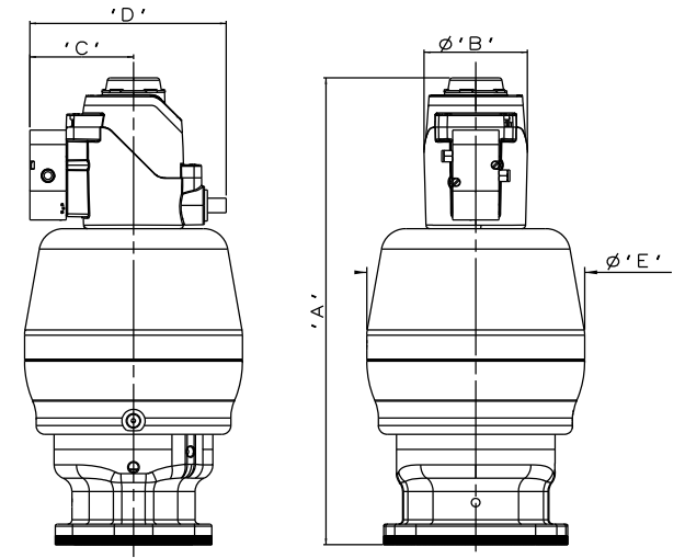
DN50 POWER S360 Ø125 PISTON SPRING CLOSING
