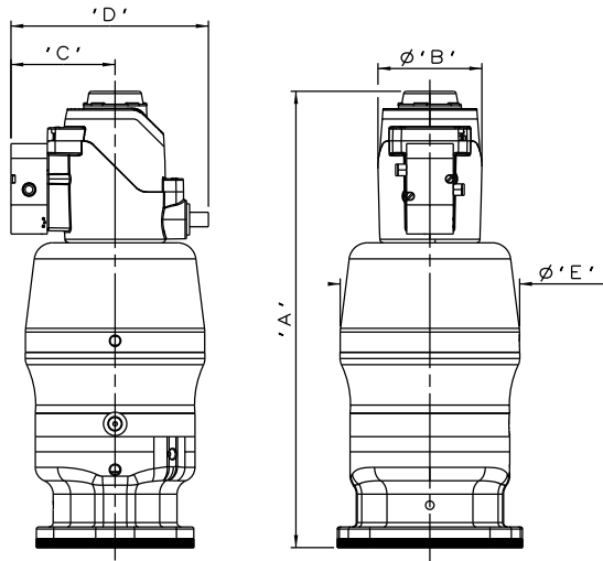
DN50 LITE S360 Ø100 PISTON SPRING CLOSING
