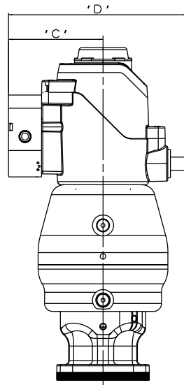
DN25 S360 \phi 80 PISTON SPRING OPENING/DOUBLE ACTING
