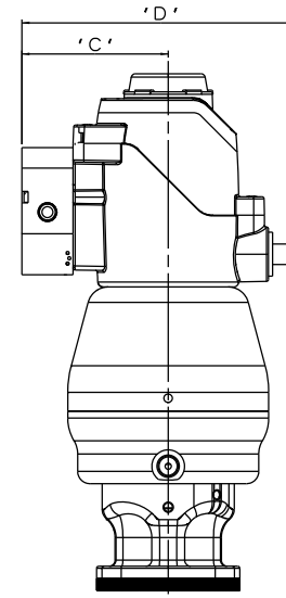
DN25 POWER S360 \phi 80 PISTON SPRING CLOSING
