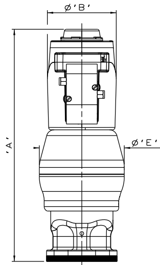
DN25 LITE S360 \phi 70 PISTON SPRING CLOSING
