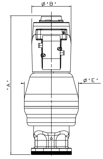
DN25 POWER S360 \phi 80 PISTON SPRING CLOSING
