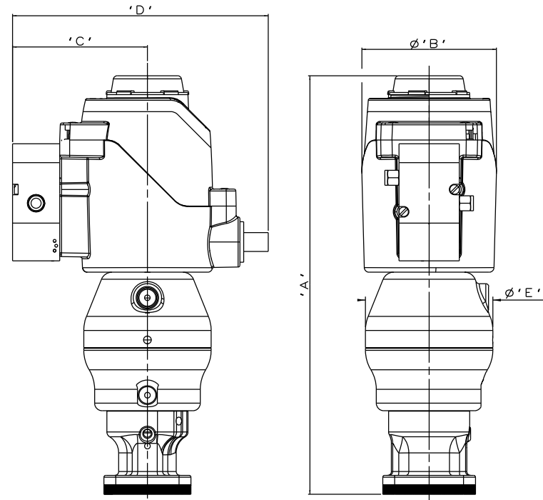
DN15 S360 ø50 PISTON SPRING OPENING/DOUBLE ACTING
