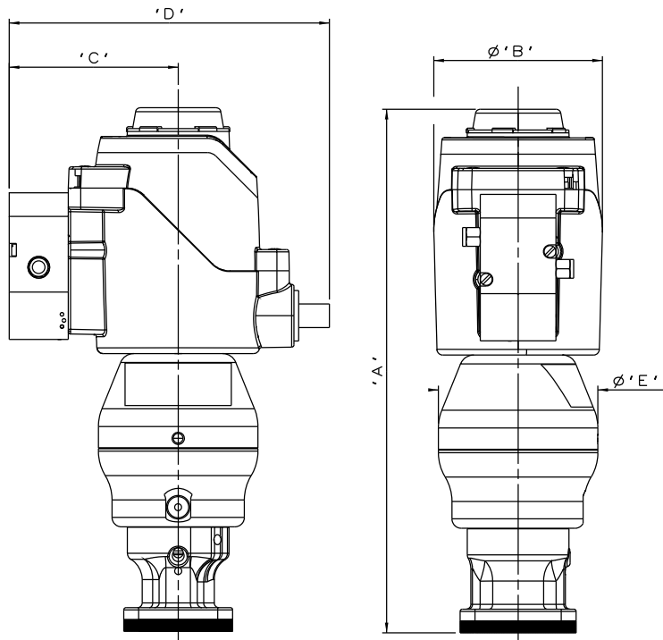
DN15 S360 ø50 PISTON SPRING CLOSING
