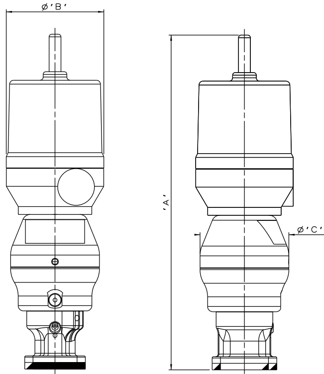
DN15 S360 \phi 50 PISTON SPRING CLOSING
