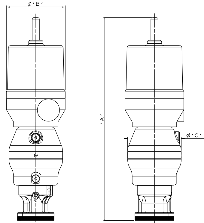
DN15 S360 \phi 50 PISTON SPRING OPENING/DOUBLE ACTING
