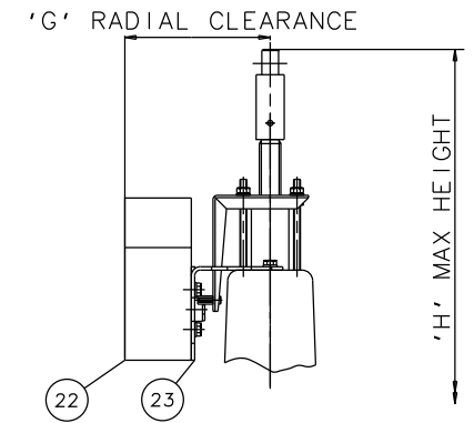
VIAPOS-MIDI POSITIONER (OPTIONAL)
