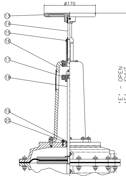
EMERGENCY HANDWHEEL (OPTIONAL)
