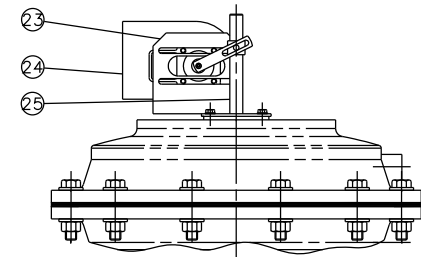
'007' SWITCHBOX (OPTIONAL)
