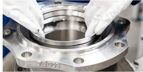
16. Using a press, apply pressure on the seat "B" (#6) to pre-compress the seat seal. Use a plastic spacer to protect the seat and apply specified pressure. In the absence of a press, contact KROMBACH for an alternative method.
