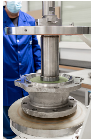
17. Insert the other seal ring (#40) over seat "B" (#6) and insert the two together into the body (#1) and over the "S" ring (#42). Apply grease to the sealing surfaces of the seat (#6). Apply pressure and axial force to pre-compress the seat seal according to the values shown in table B and in the same manner as done on the cover (tail) side.
